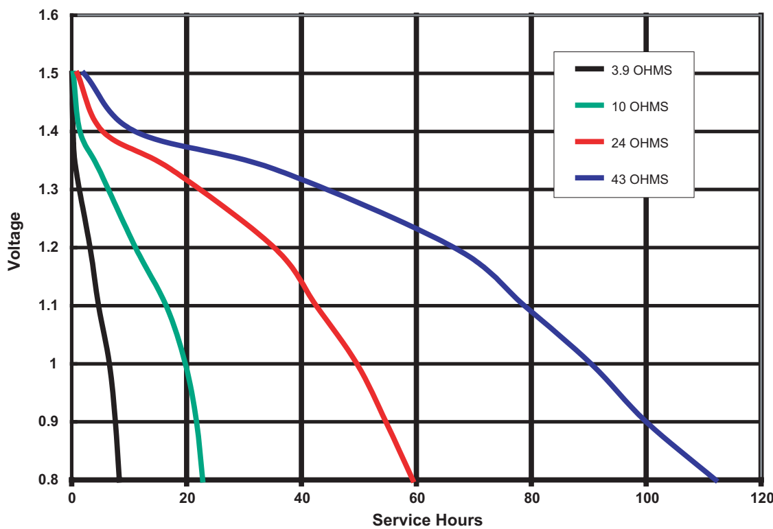
TYPICAL DISCHARGE CHARACTERISTICS AT 21°C (70°F)
