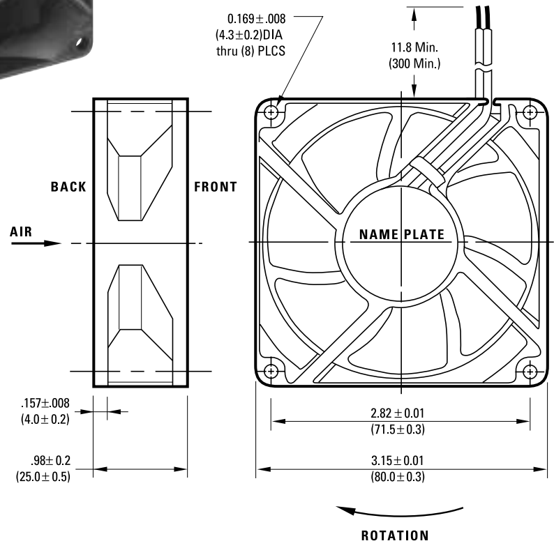
FLANGE TYPE (P00)
